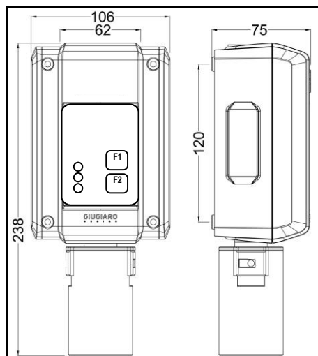
Fig. 1 – Dimensioni / Size / Dimensions
